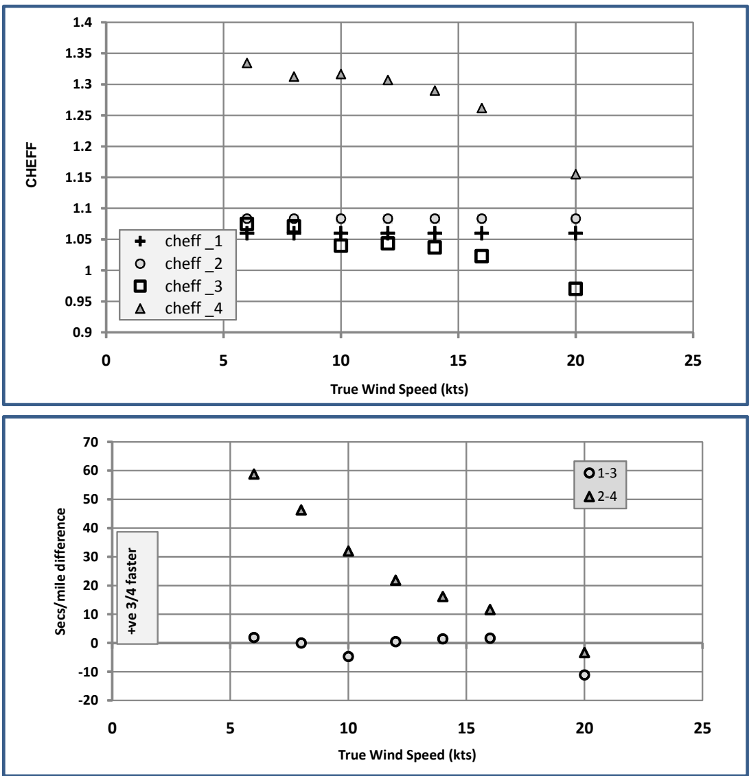
Figure 4.3 – Effective rig height factor vs. True wind speed for 85% and 100% fractionality.
